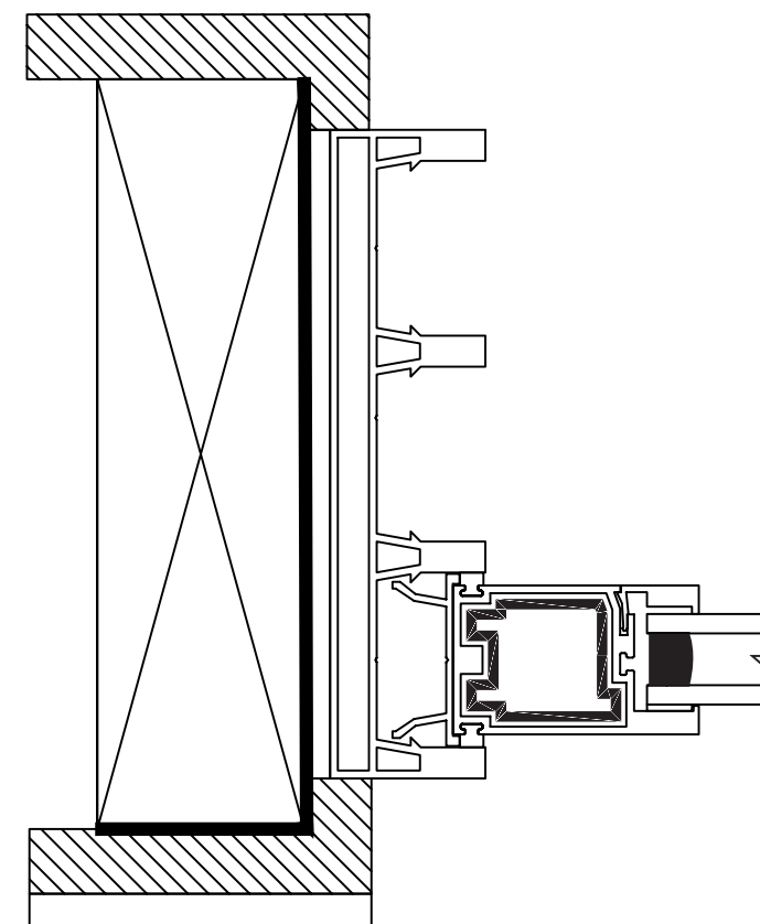
Outside of Structure Jamb Horizontal Section 3-Track 2x8 Equal Leg
