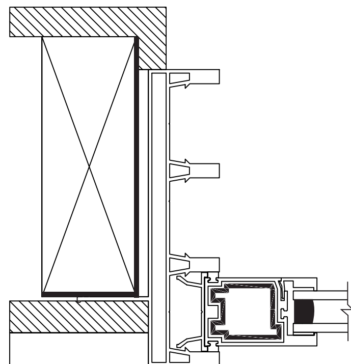
Outside of Structure Jamb Horizontal Section 3-Track 2x6 1.375" Nail Fin
