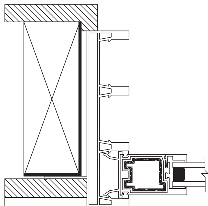
Outside of Structure Jamb Horizontal Section 3-Track 2x6 1" Nail Fin
